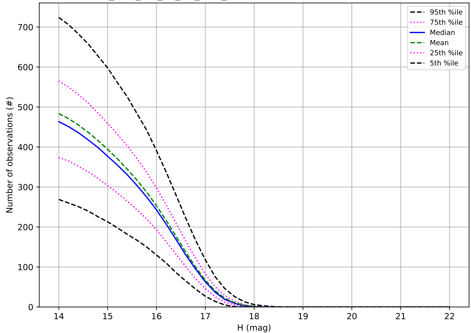
too_elab_r32_d3_giz_v3.4_10yrs: Number of observations Trojan
