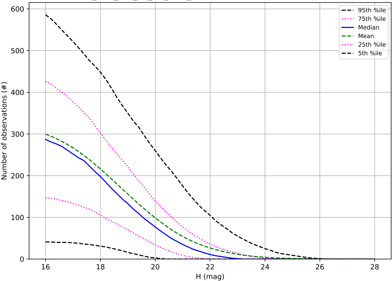
too_elab_r32_d3_giz_v3.4_10yrs: Number of observations PHA
