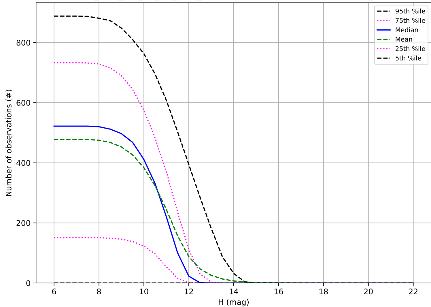
too_elab_r32_d3_giz_v3.4_10yrs: Number of observations OCC_r20
