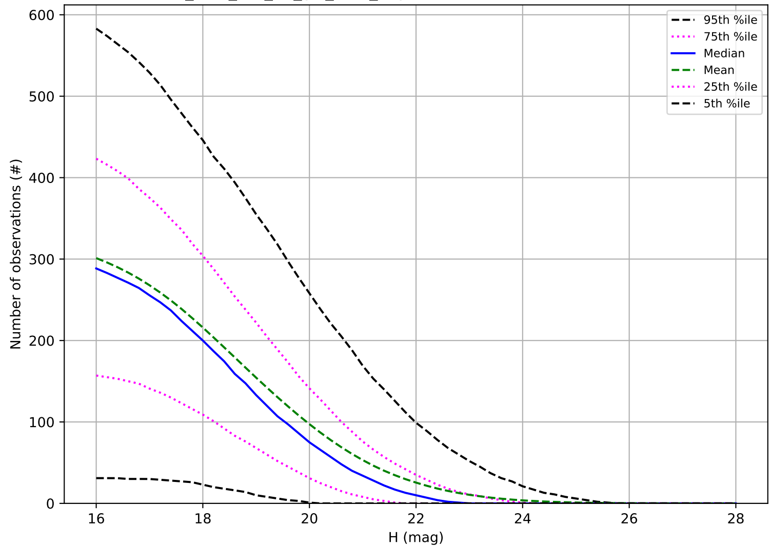
too_elab_r32_d3_giz_v3.4_10yrs: Number of observations NEO
