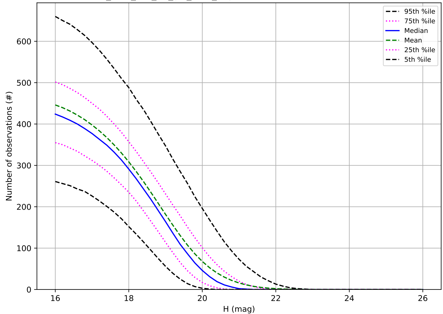
too_elab_r32_d3_giz_v3.4_10yrs: Number of observations MBA
