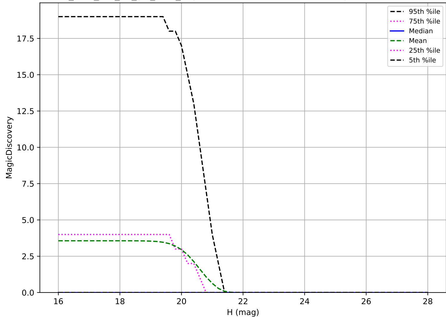
too_elab_r32_d3_giz_v3.4_10yrs: Vatira 6 detections in 60 nights detection loss
