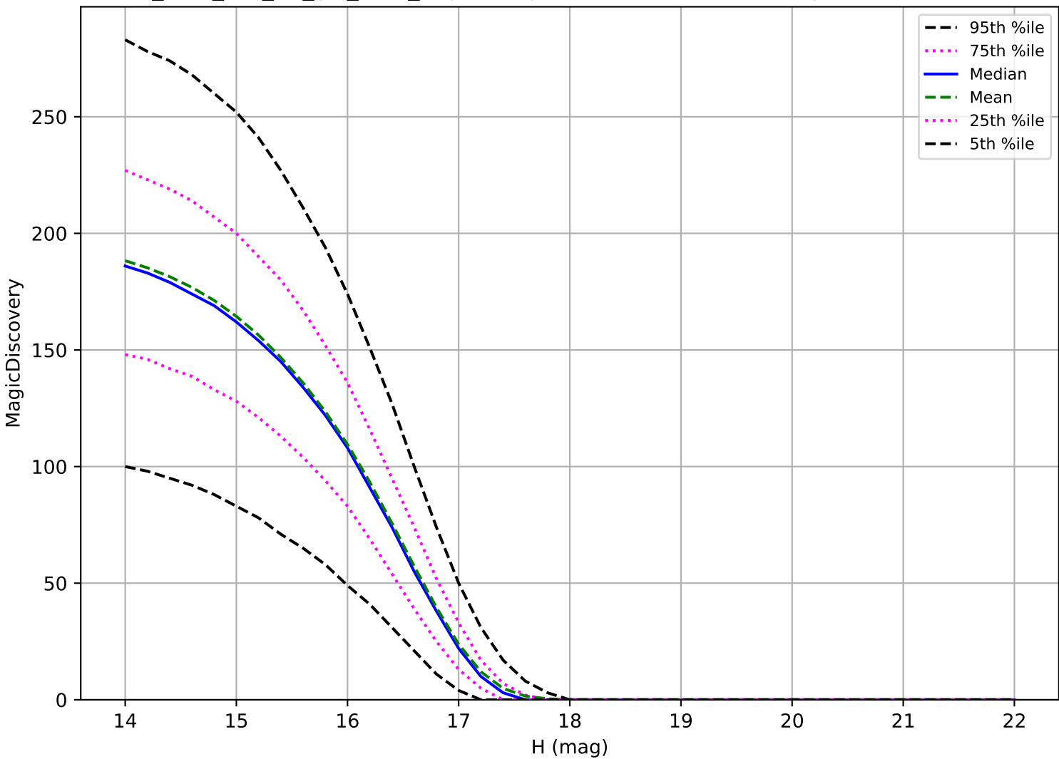
too_elab_r32_d3_giz_v3.4_10yrs: Trojan 6 detections in 60 nights detection loss
