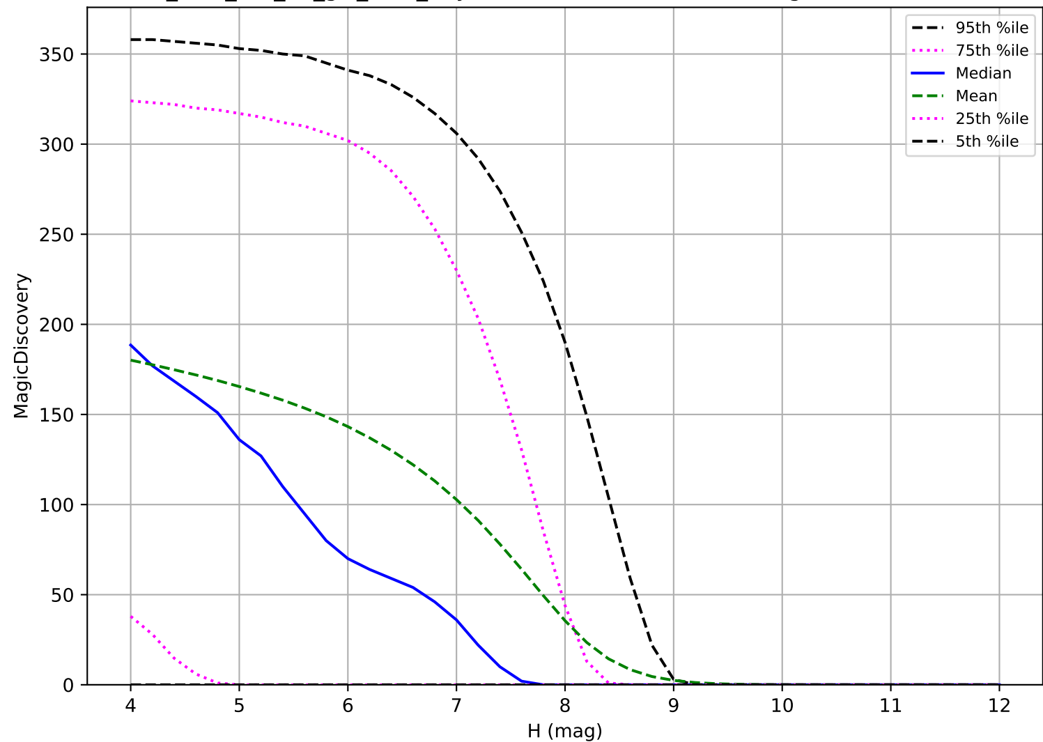
too_elab_r32_d3_giz_v3.4_10yrs: TNO 6 detections in 60 nights detection loss
