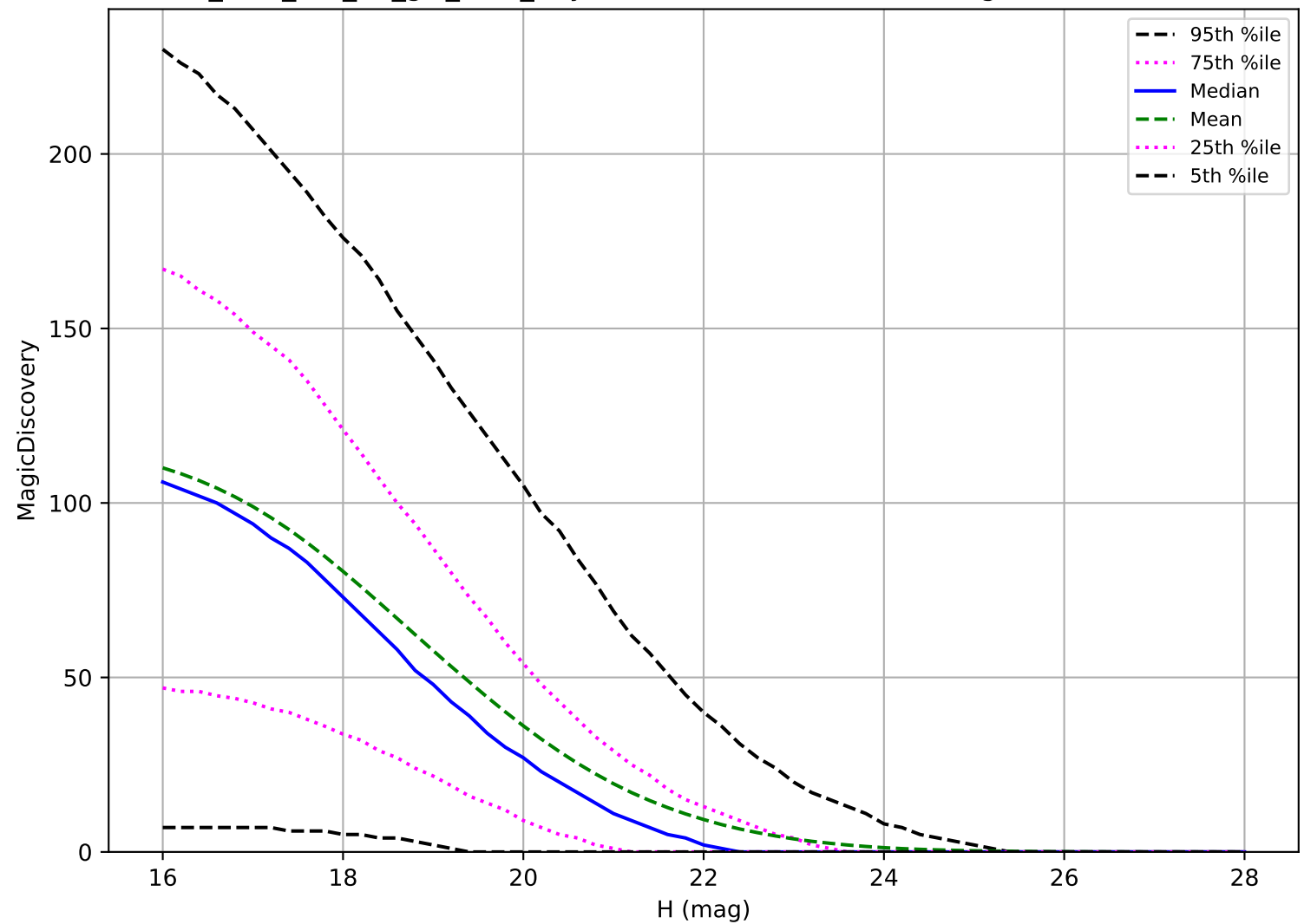
too_elab_r32_d3_giz_v3.4_10yrs: PHA 6 detections in 60 nights detection loss
