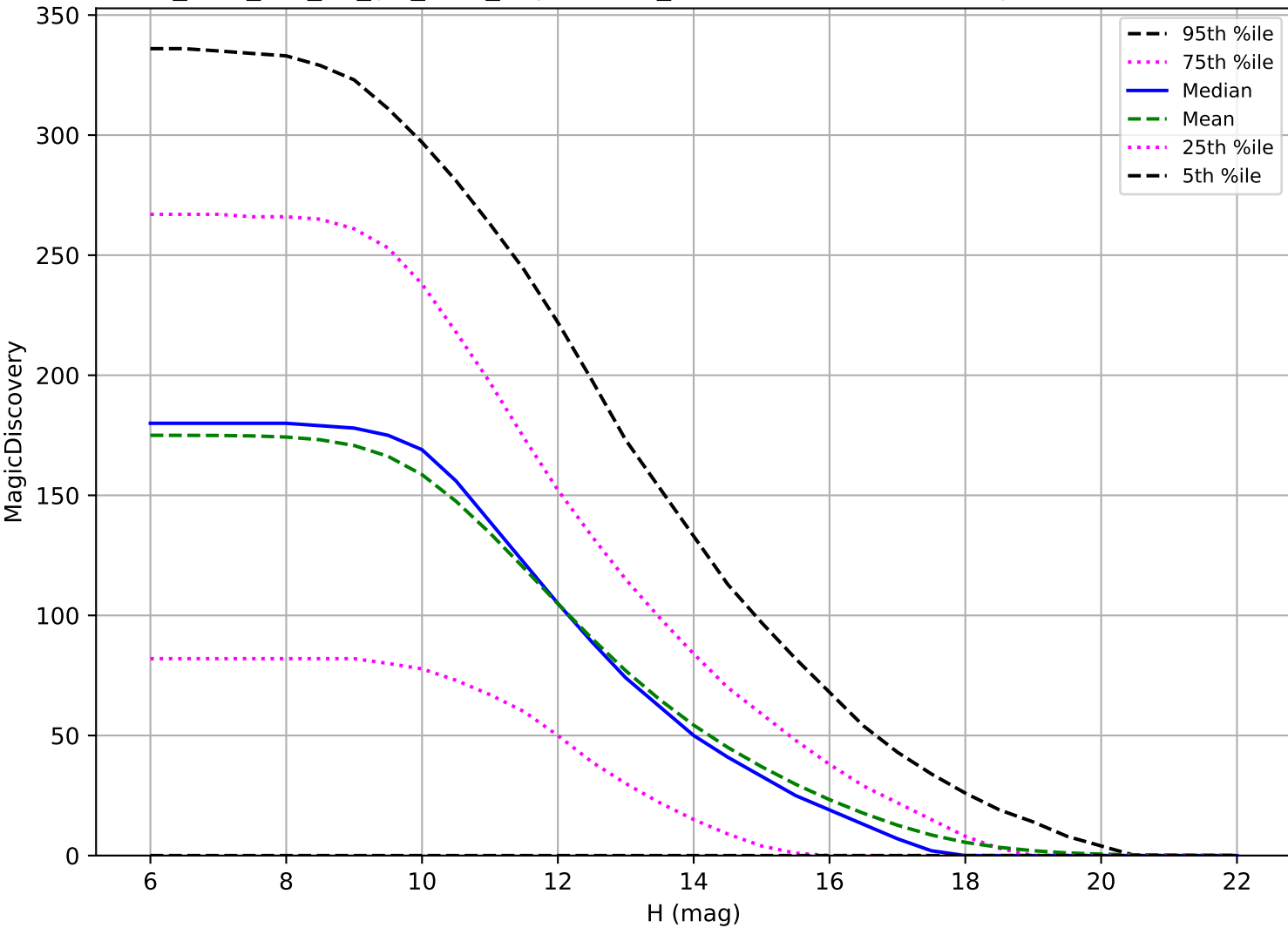
too_elab_r32_d3_giz_v3.4_10yrs: OCC_r5 6 detections in 60 nights detection loss
