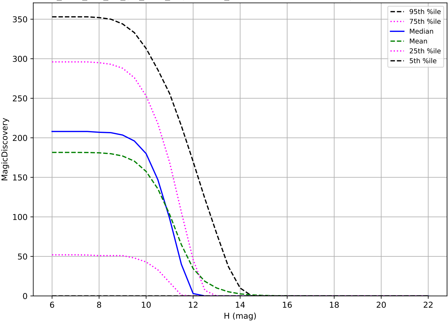
too_elab_r32_d3_giz_v3.4_10yrs: OCC_r20 6 detections in 60 nights detection loss
