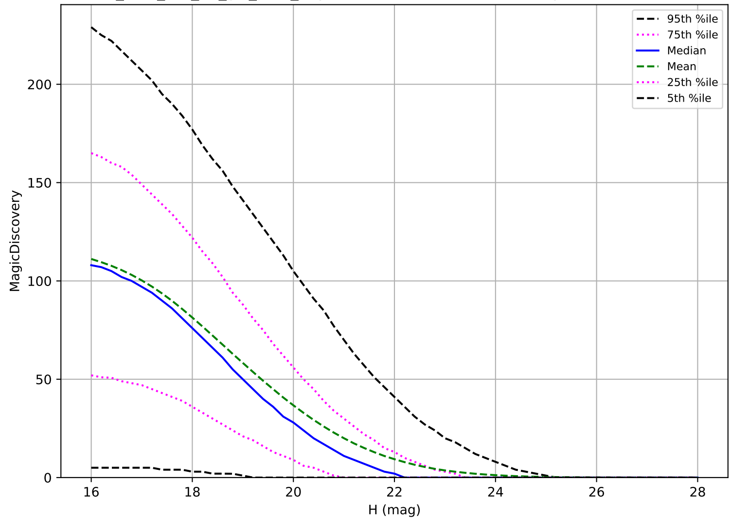
too_elab_r32_d3_giz_v3.4_10yrs: NEO 6 detections in 60 nights detection loss
