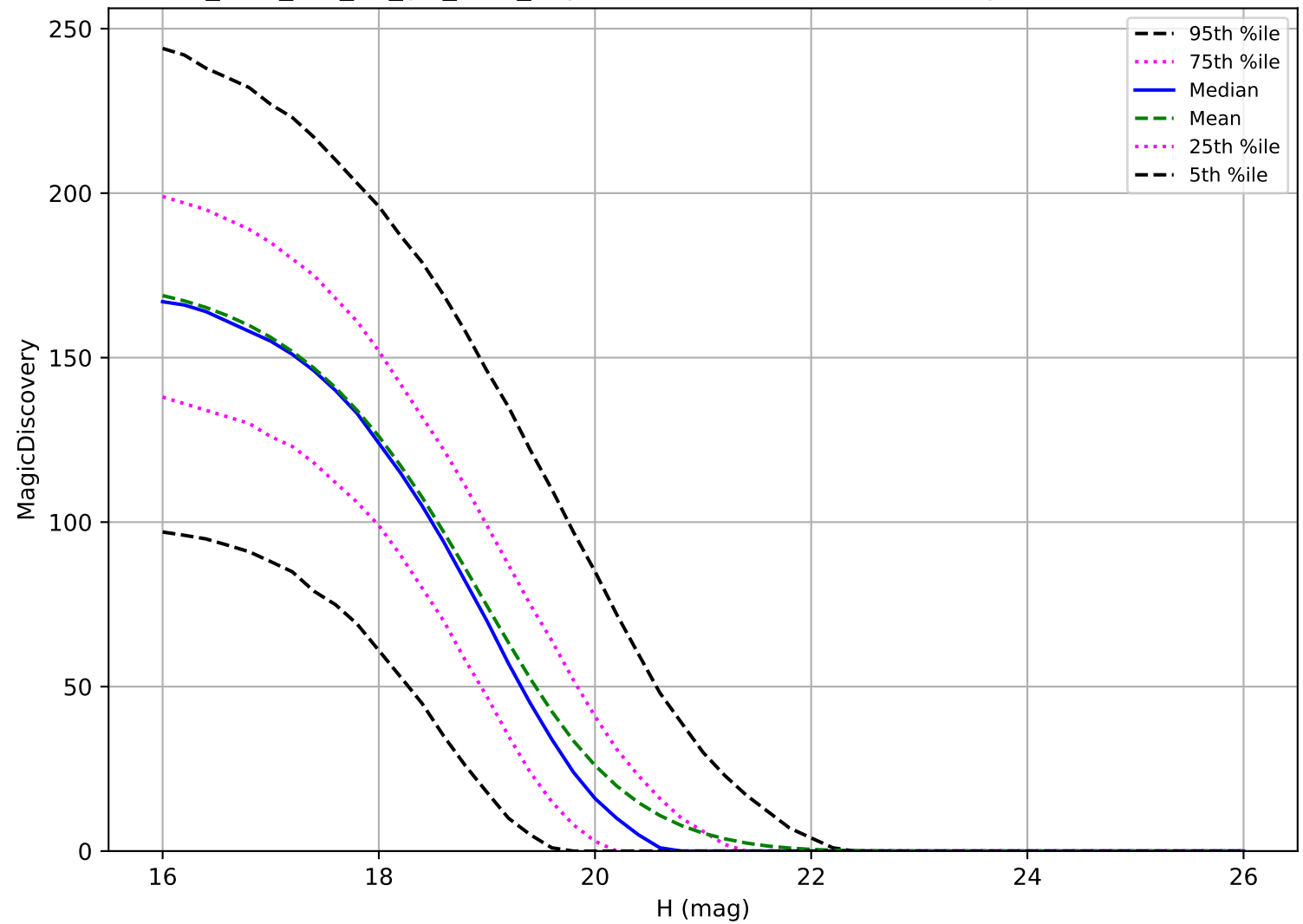
too_elab_r32_d3_giz_v3.4_10yrs: MBA 6 detections in 60 nights detection loss
