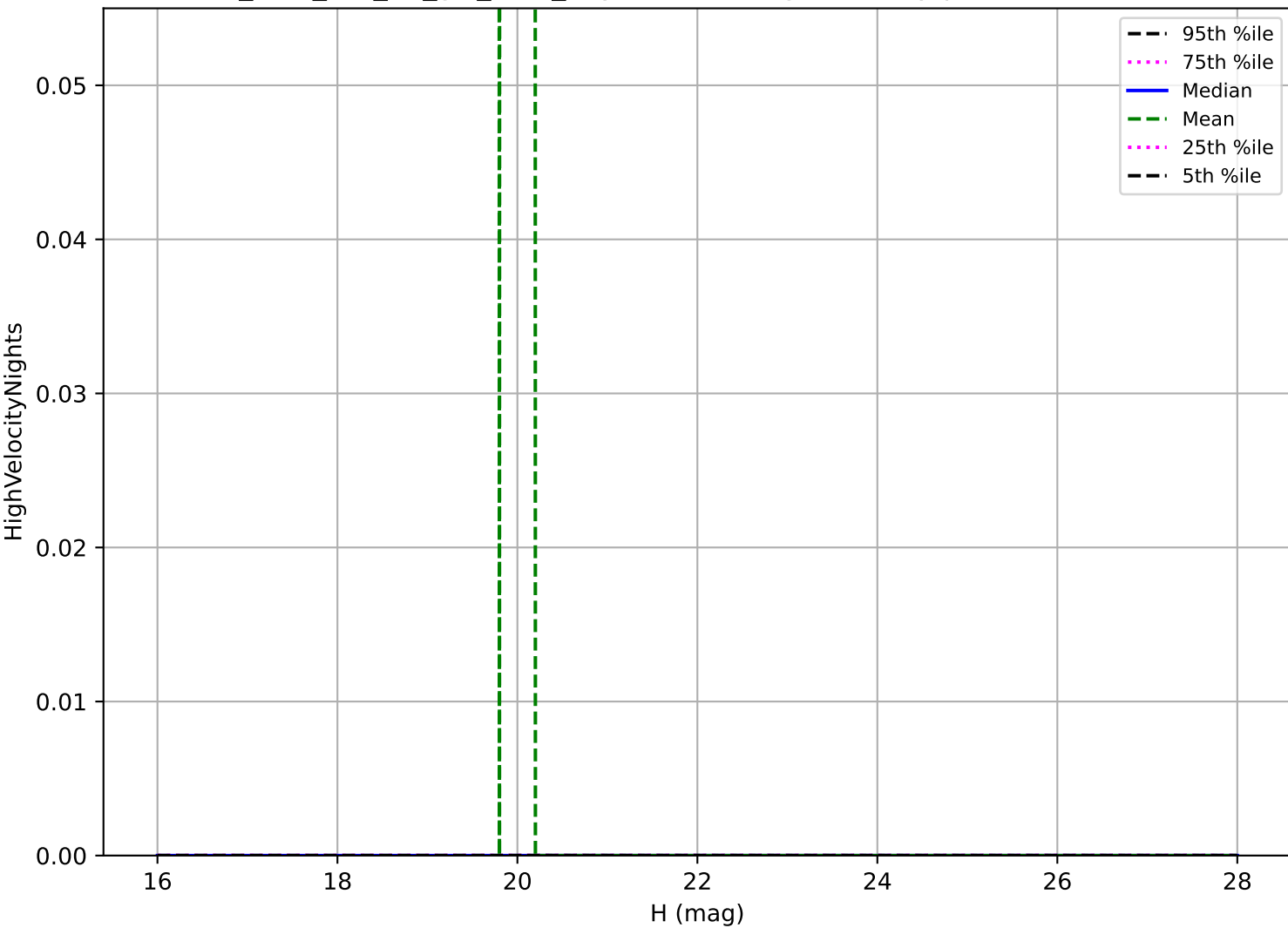
too_elab_r32_d3_giz_v3.4_10yrs: Vatira High velocity pair detection loss
