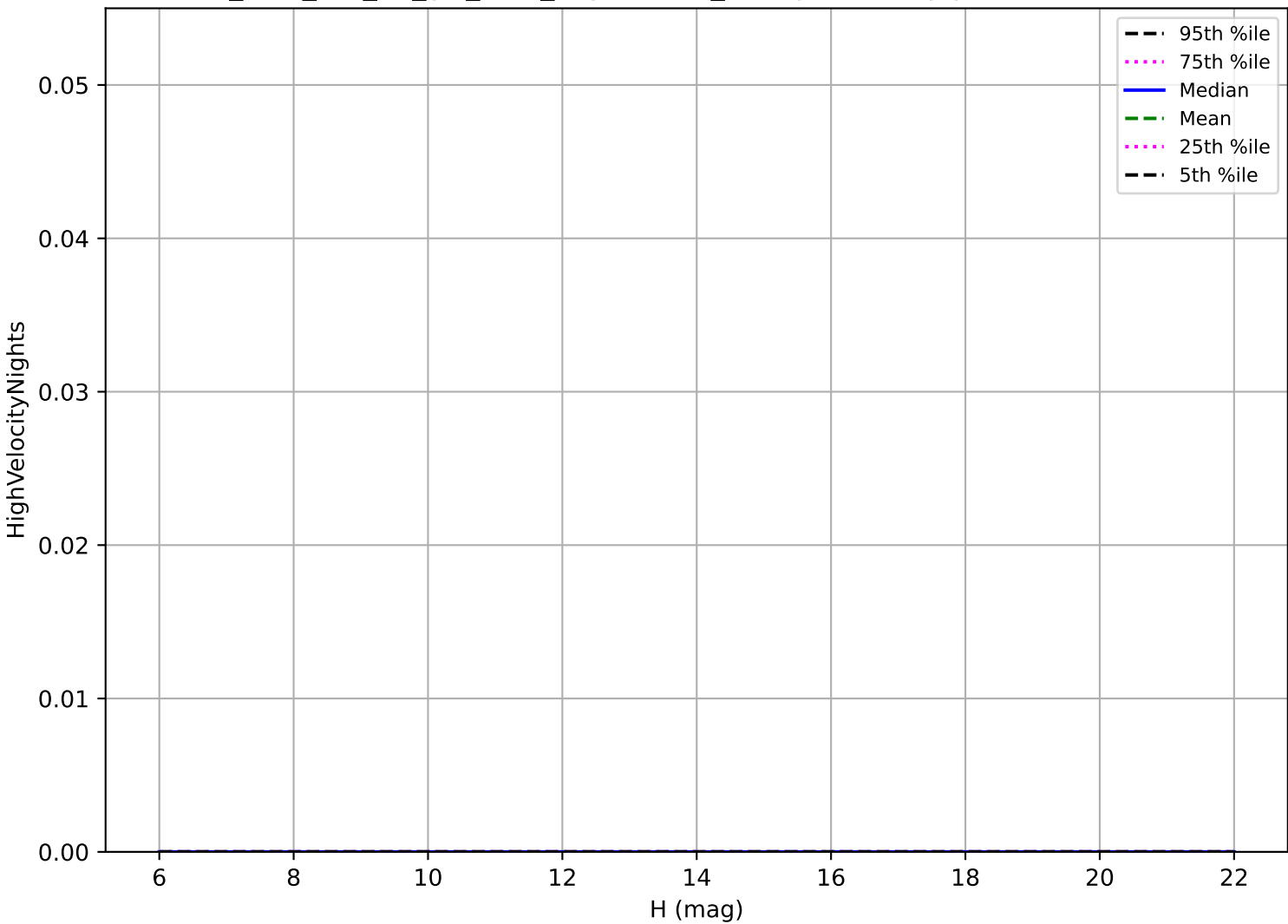
too_elab_r32_d3_giz_v3.4_10yrs: OCC_r5 High velocity pair detection loss
