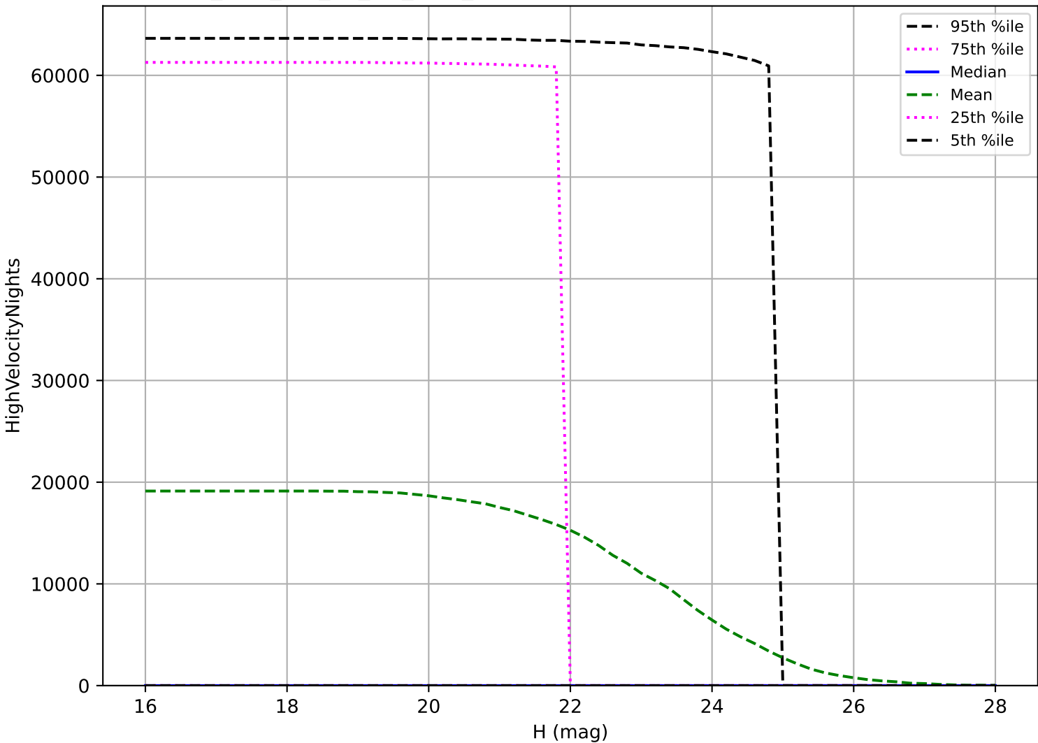
too_elab_r32_d3_giz_v3.4_10yrs: NEO High velocity pair detection loss
