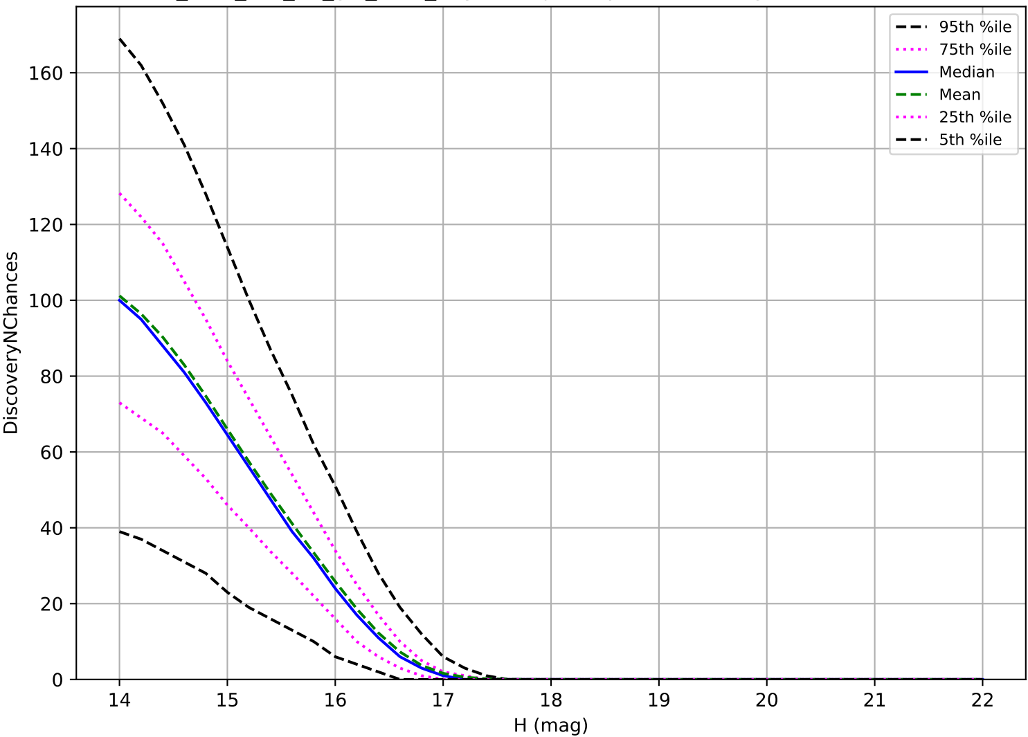
too_elab_r32_d3_giz_v3.4_10yrs: Trojan 3 pairs in 15 nights detection loss
