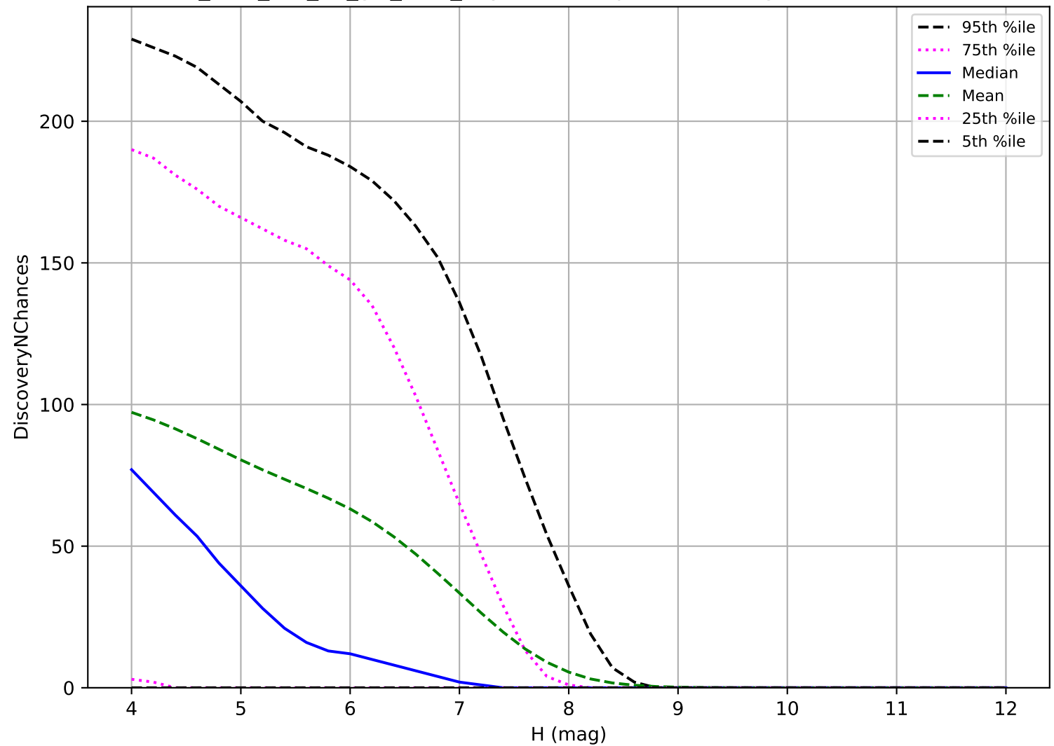
too_elab_r32_d3_giz_v3.4_10yrs: TNO 3 pairs in 15 nights detection loss
