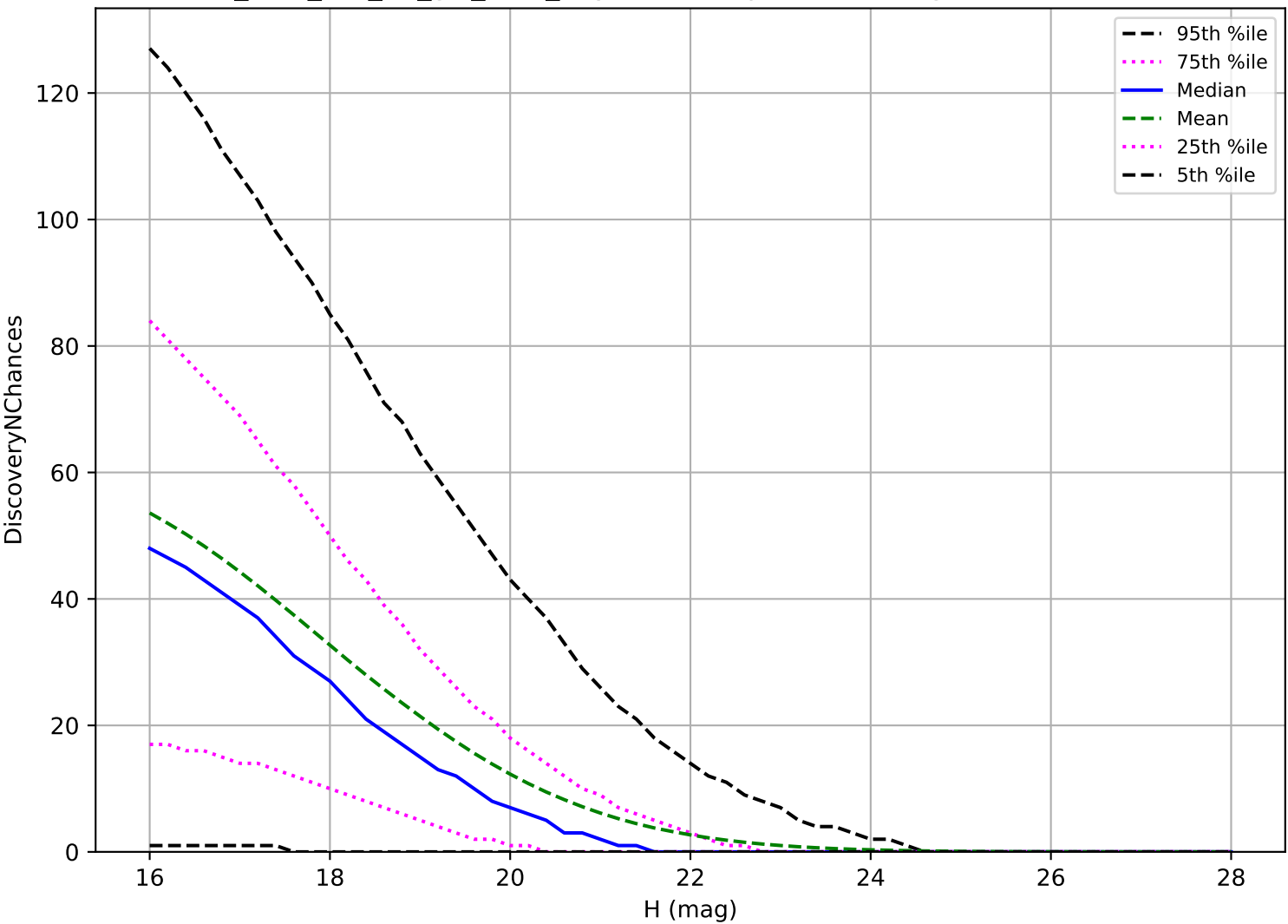
too_elab_r32_d3_giz_v3.4_10yrs: PHA 3 pairs in 15 nights detection loss
