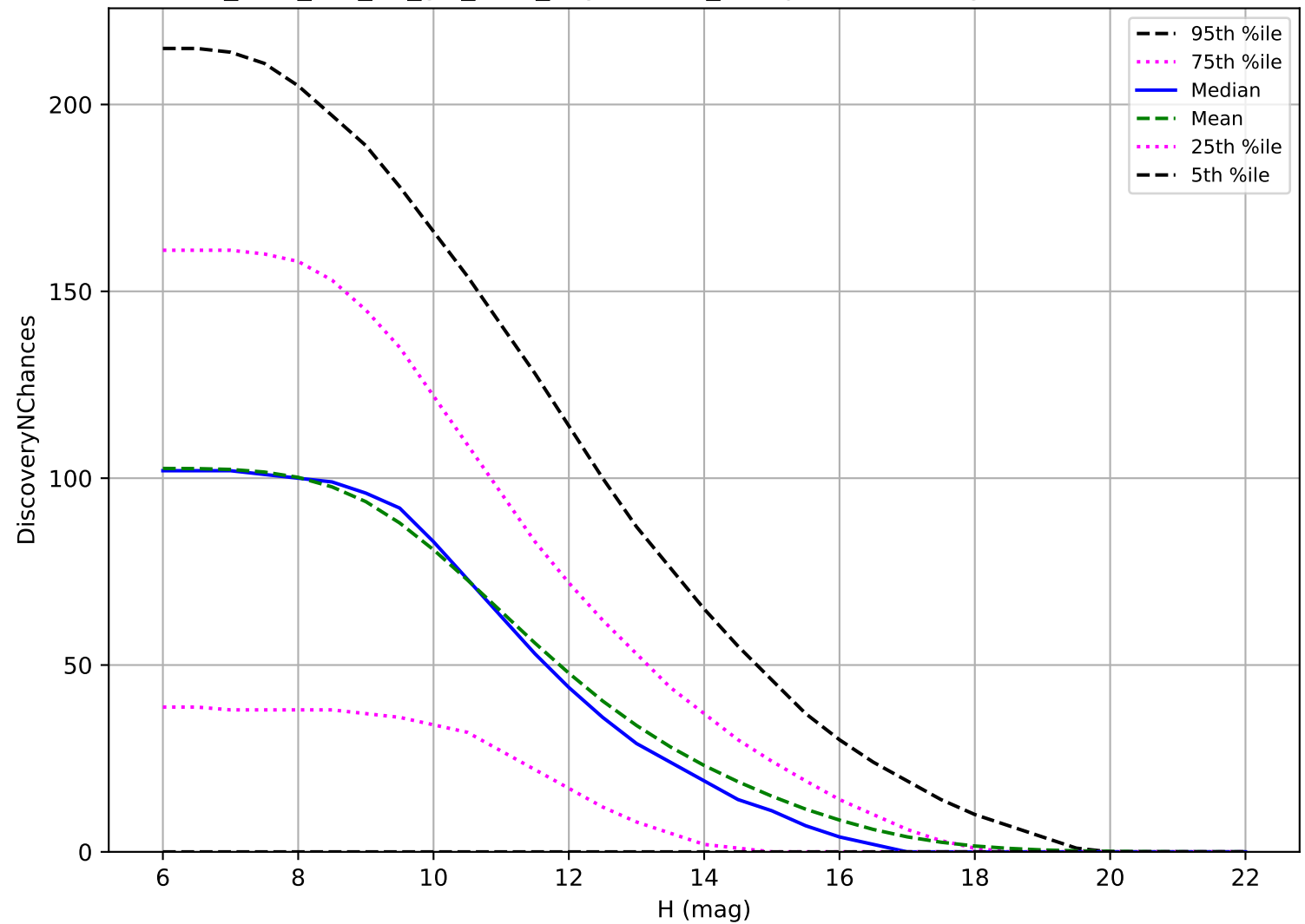
too_elab_r32_d3_giz_v3.4_10yrs: OCC_r5 3 pairs in 15 nights detection loss
