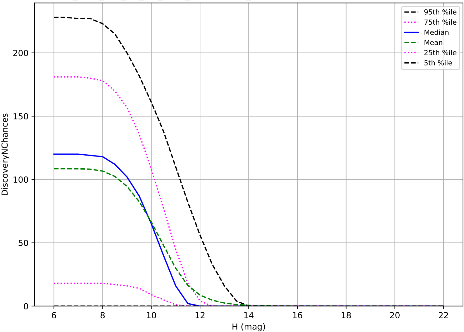
too_elab_r32_d3_giz_v3.4_10yrs: OCC_r20 3 pairs in 15 nights detection loss
