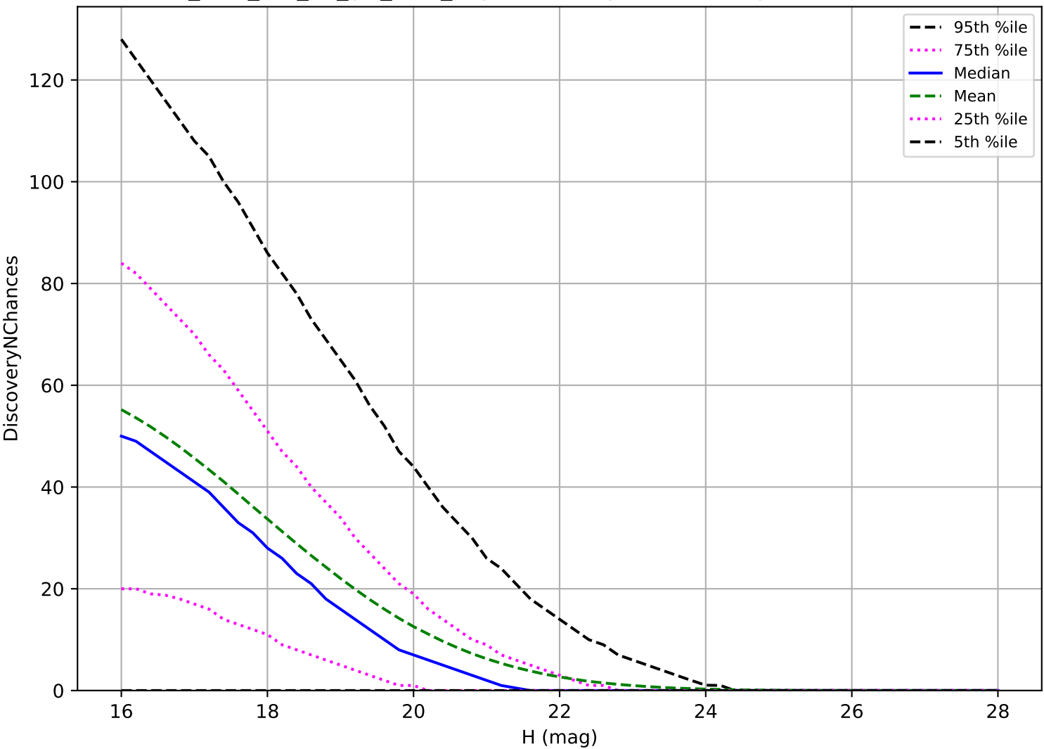
too_elab_r32_d3_giz_v3.4_10yrs: NEO 3 pairs in 15 nights detection loss
