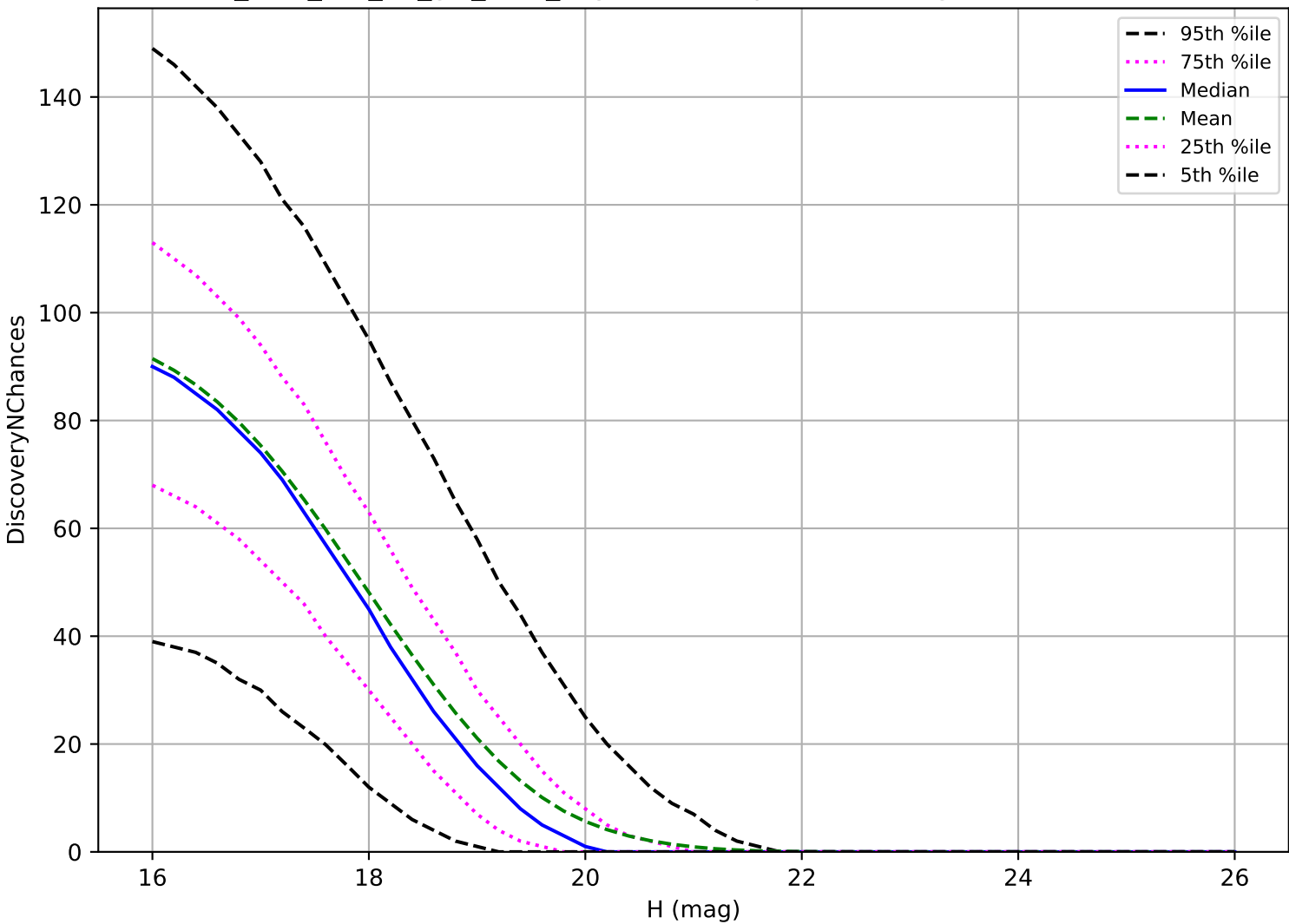
too_elab_r32_d3_giz_v3.4_10yrs: MBA 3 pairs in 15 nights detection loss
