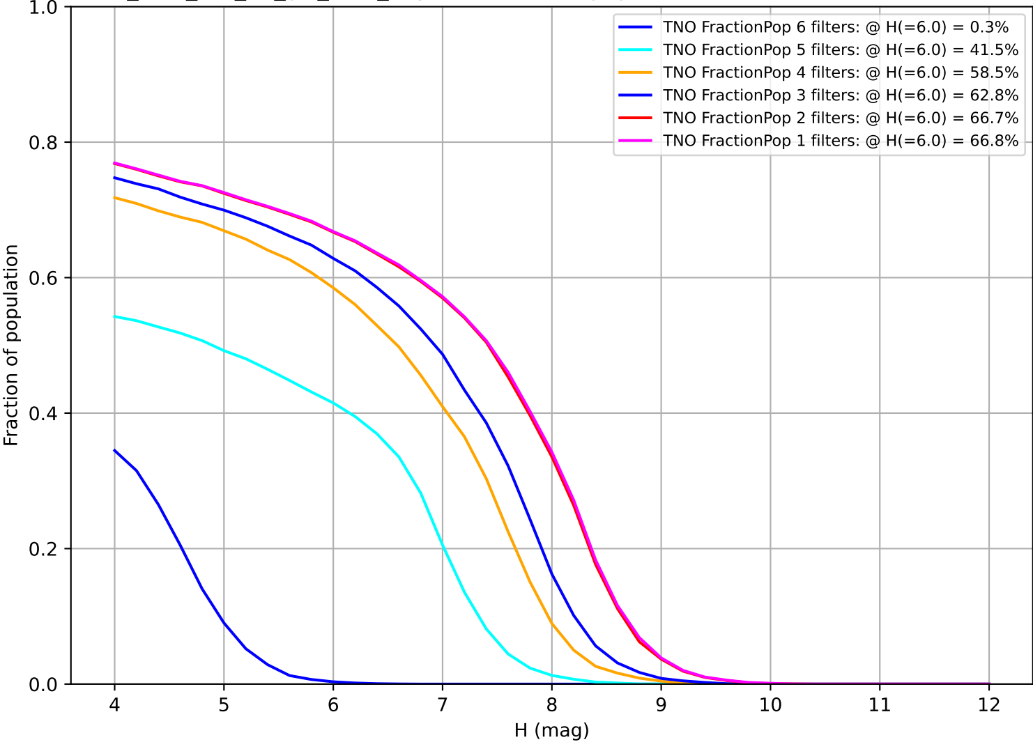
too_elab_r32_d3_giz_v3.4_10yrs: Fraction of population with colors in X filters TNO
