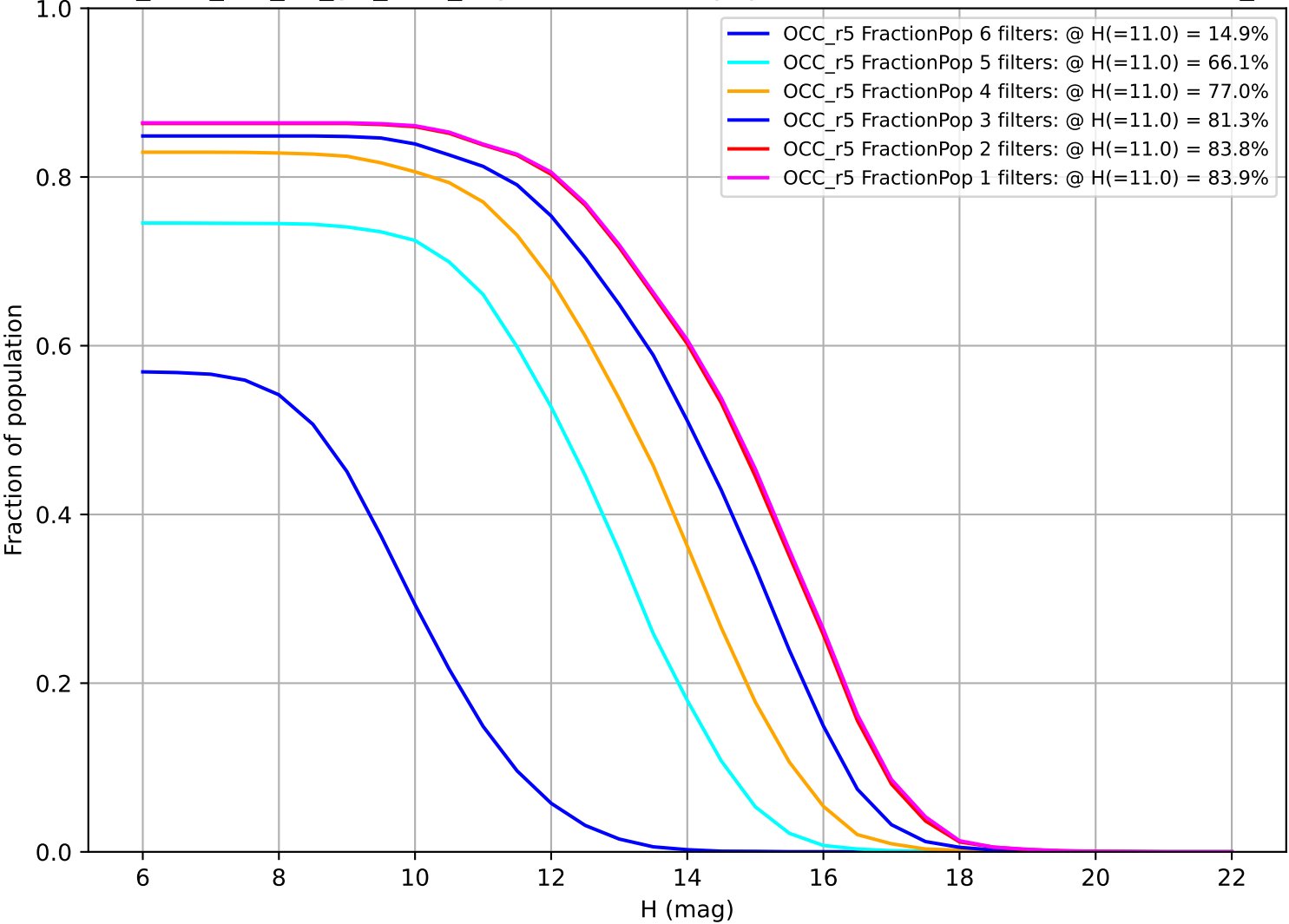
too_elab_r32_d3_giz_v3.4_10yrs: Fraction of population with colors in X filters OCC_r5
