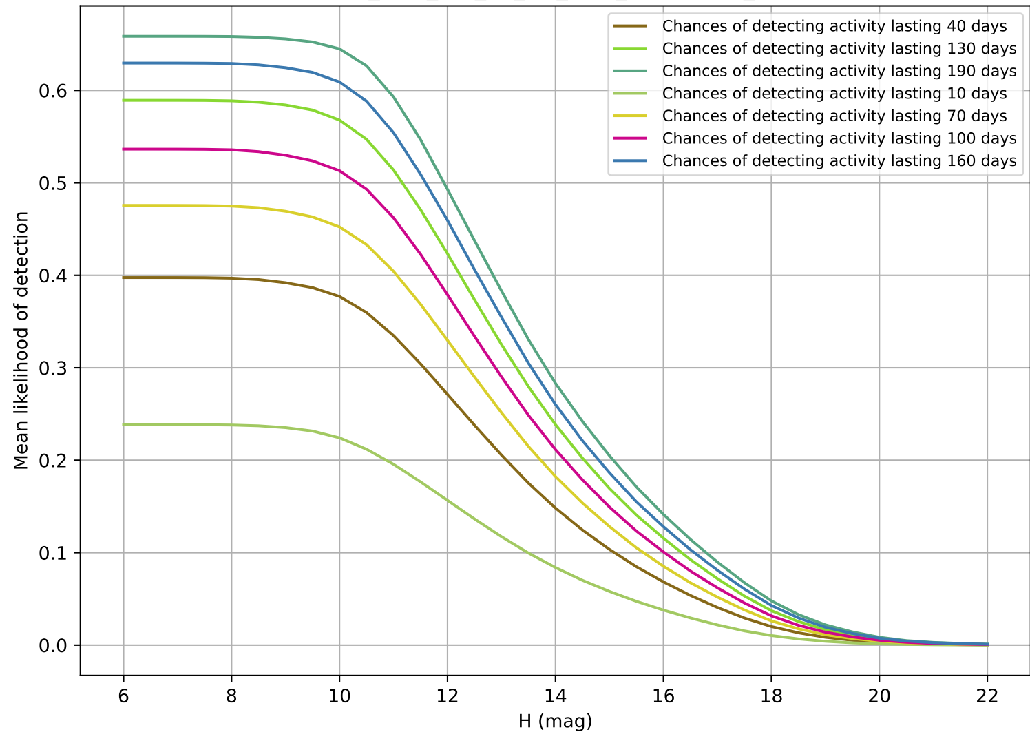
too_elab_r32_d3_giz_v3.4_10yrs OCC_r5
