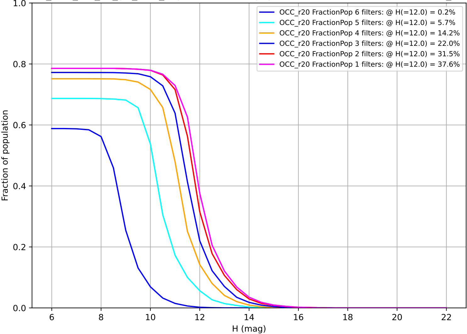
too_elab_r32_d3_giz_v3.4_10yrs: Fraction of population with colors in X filters OCC_r20
