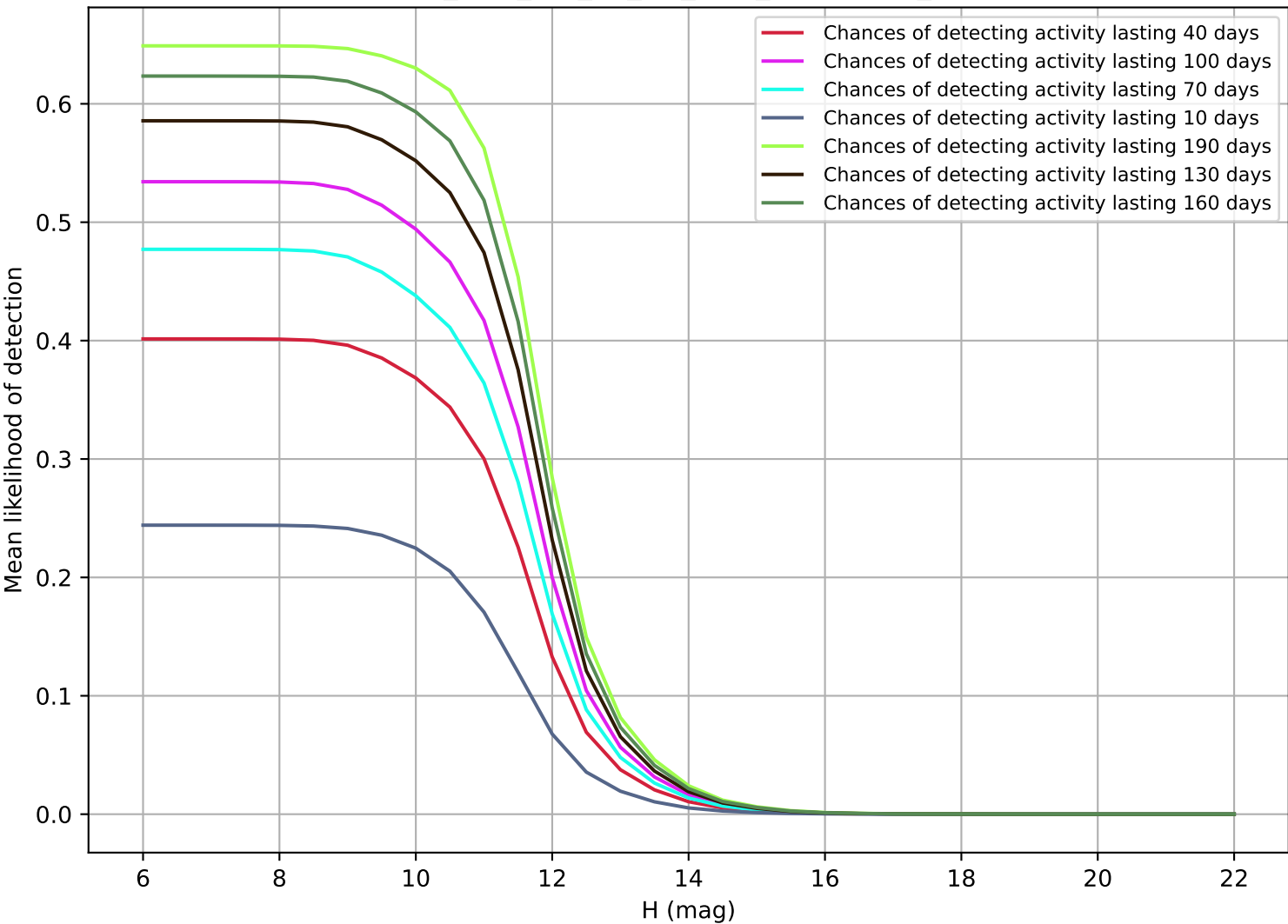
too_elab_r32_d3_giz_v3.4_10yrs OCC_r20
