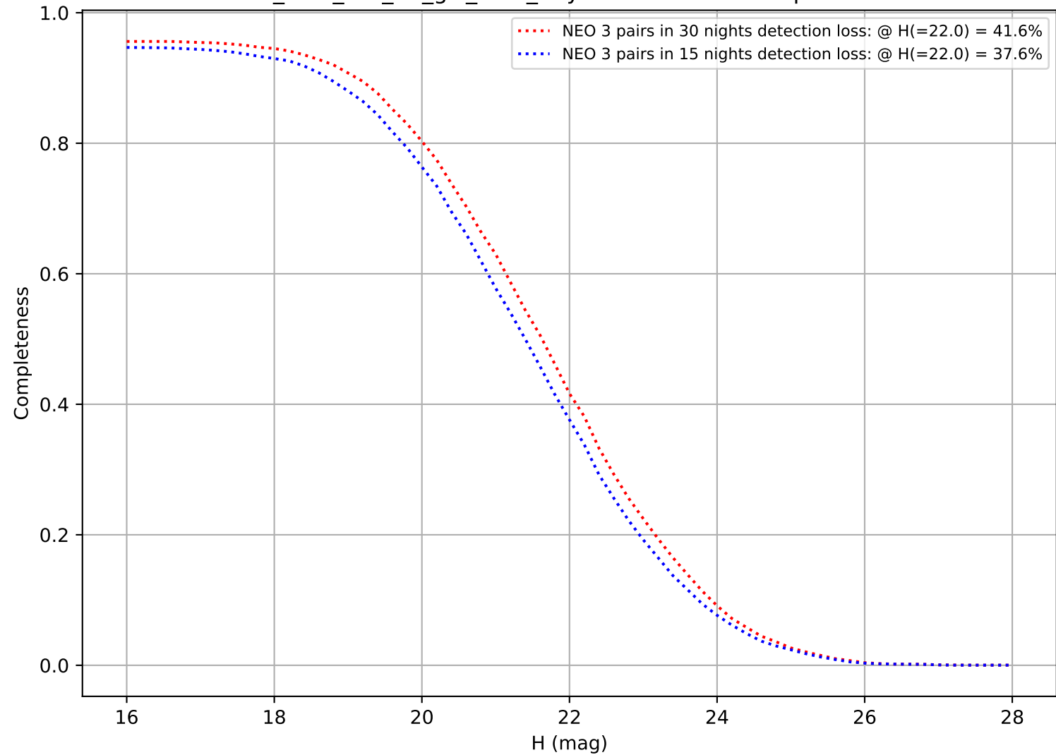
too_elab_r32_d3_giz_v3.4_10yrs: DifferentialCompleteness
