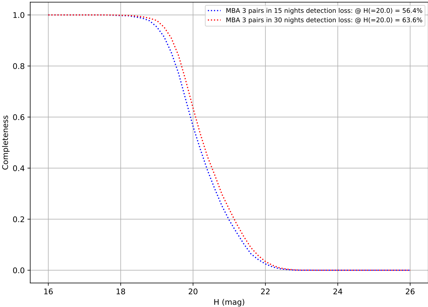
too_elab_r32_d3_giz_v3.4_10yrs: DifferentialCompleteness
