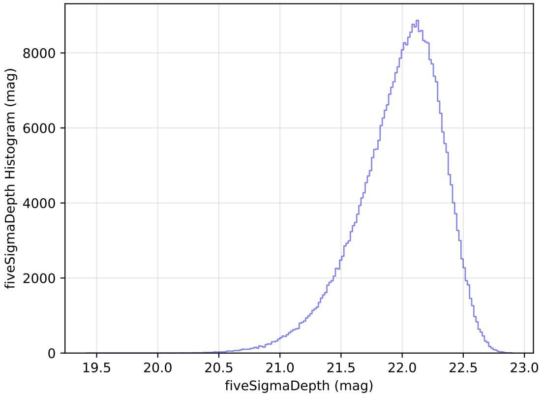
too_elab_r32_d3_giz_v3.4_10yrs y: fiveSigmaDepth Histogram
