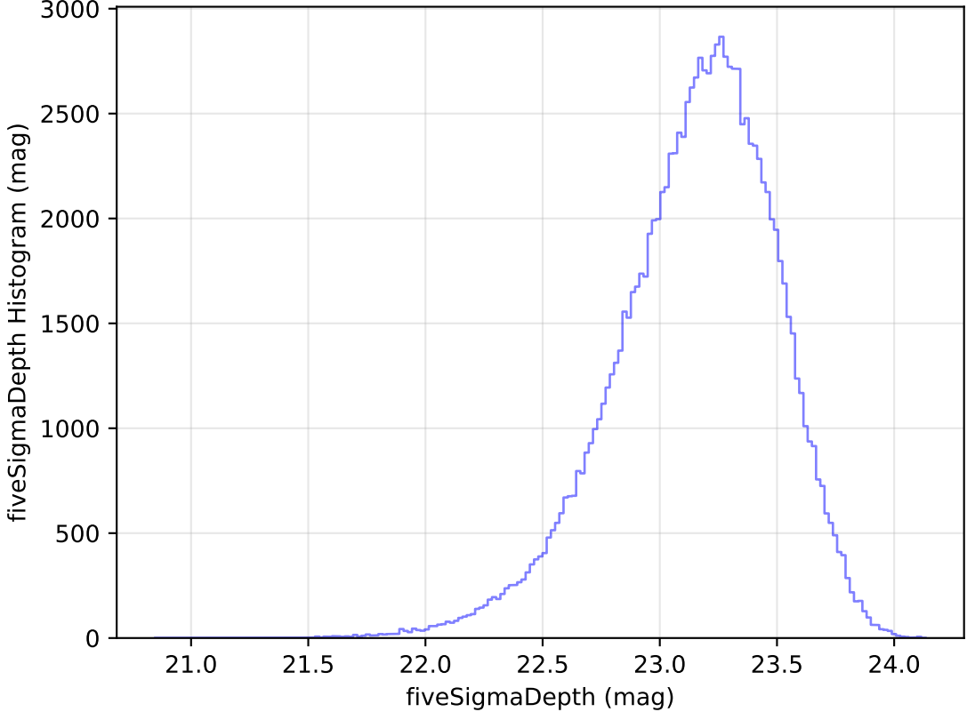
too_elab_r32_d3_giz_v3.4_10yrs u: fiveSigmaDepth Histogram
