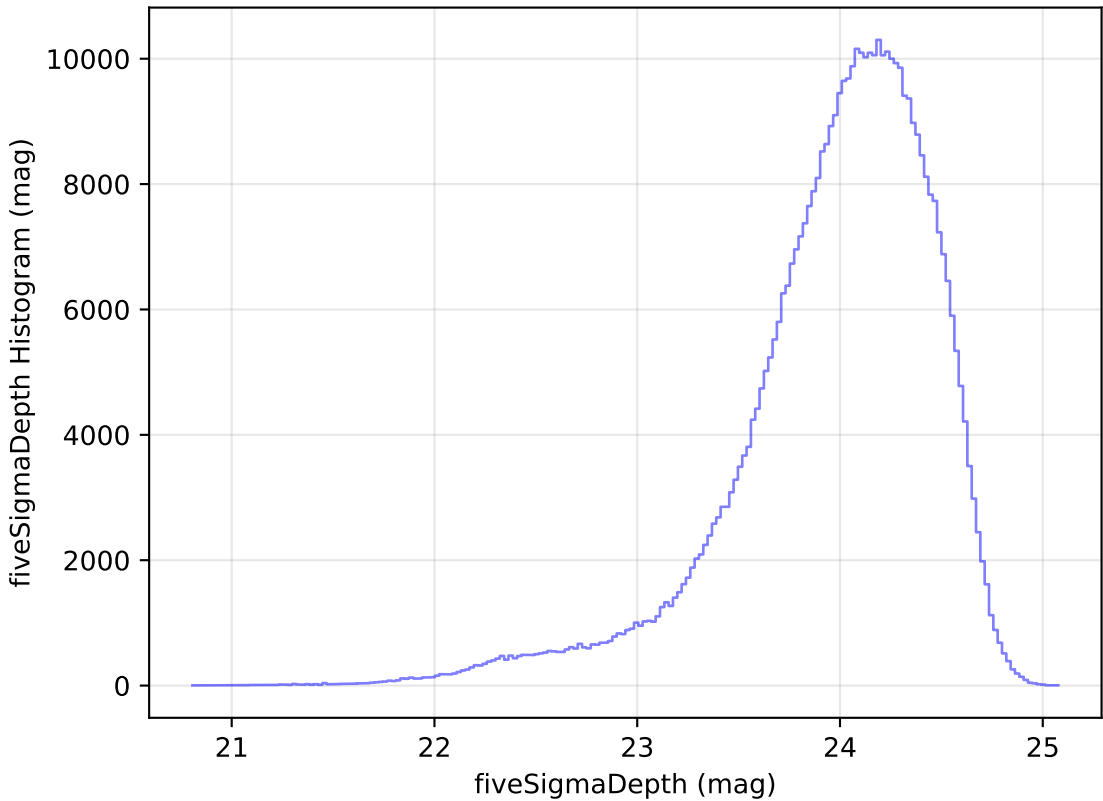
too_elab_r32_d3_giz_v3.4_10yrs r: fiveSigmaDepth Histogram
