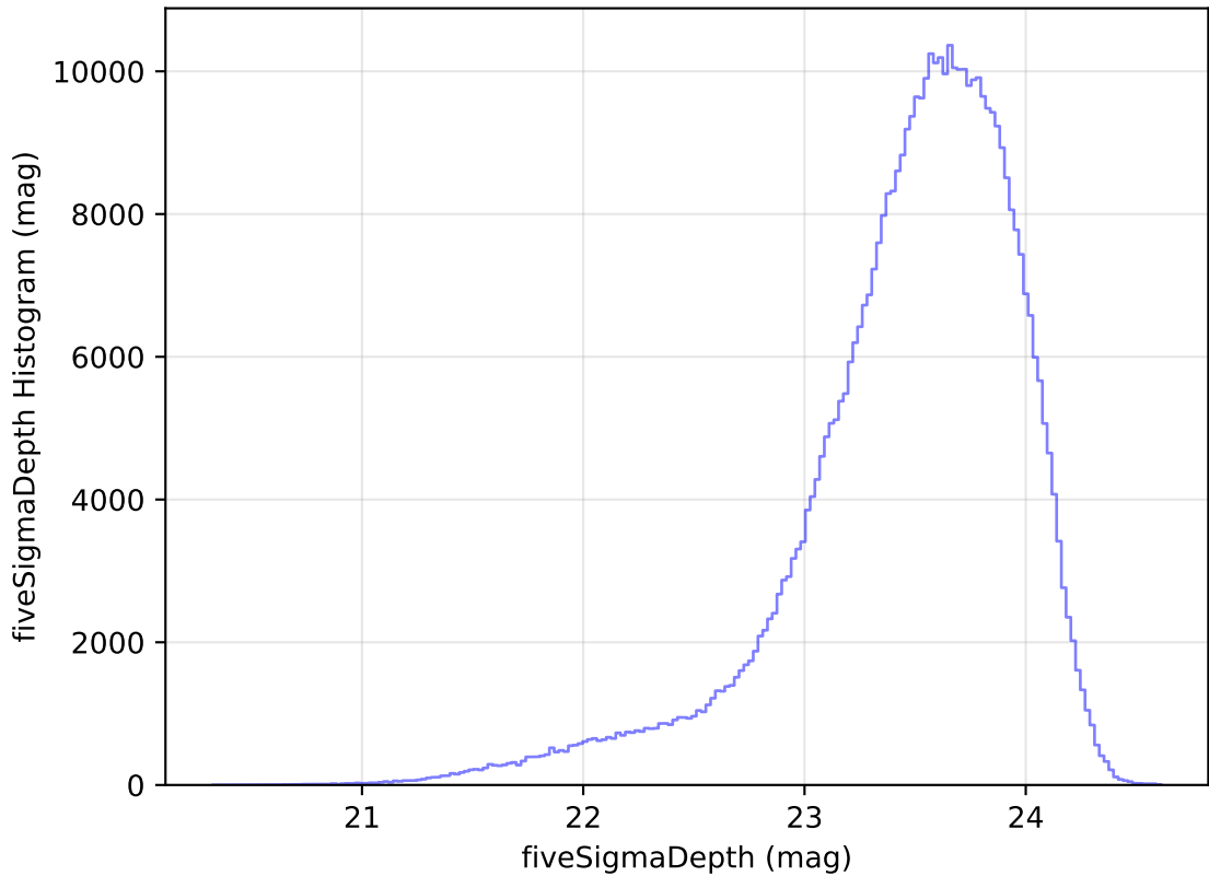
too_elab_r32_d3_giz_v3.4_10yrs i: fiveSigmaDepth Histogram
