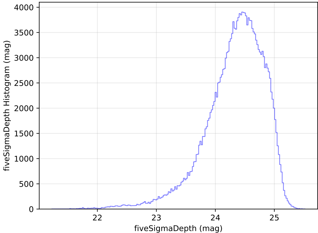
too_elab_r32_d3_giz_v3.4_10yrs g: fiveSigmaDepth Histogram
