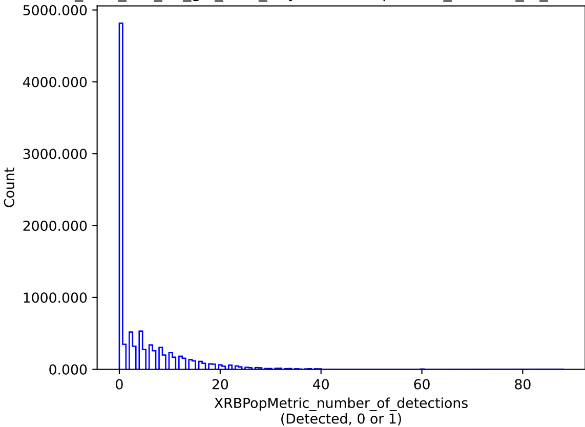
too_elab_r32_d3_giz_v3.4_10yrs : XRBPoMetric_number_of_detections
