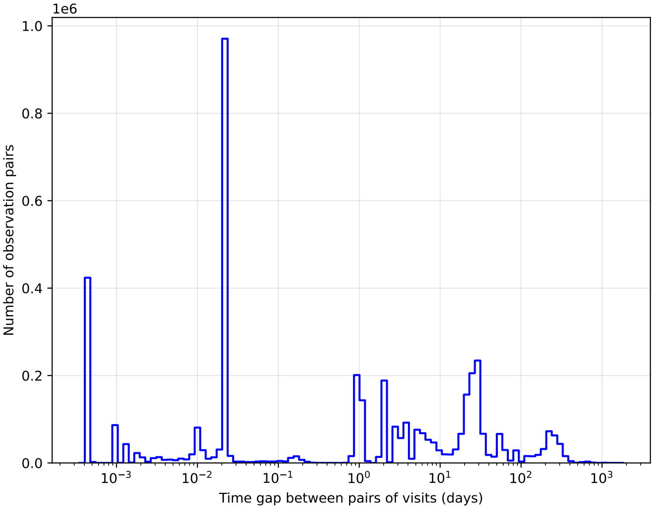
too_elab_r32_d3_giz_v3.4_10yrs y band: Tgaps observationStartMJD
