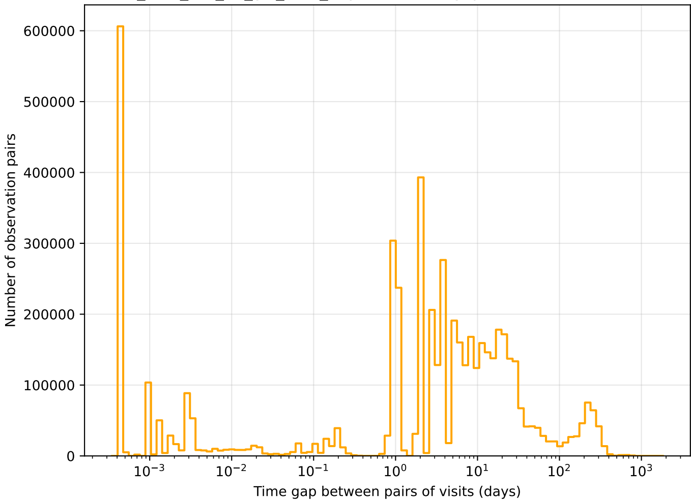
too_elab_r32_d3_giz_v3.4_10yrs r band: Tgaps observationStartMJD
