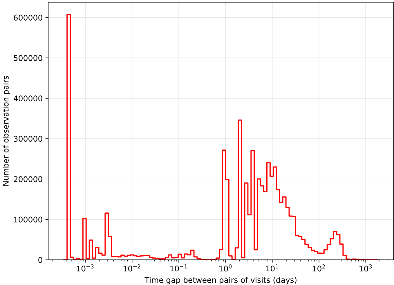
too_elab_r32_d3_giz_v3.4_10yrs i band: Tgaps observationStartMJD
