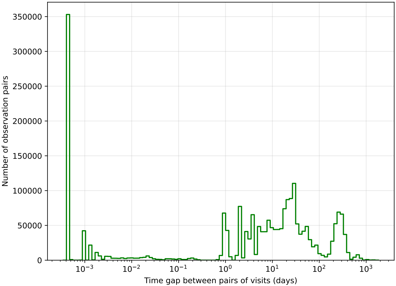
too_elab_r32_d3_giz_v3.4_10yrs g band: Tgaps observationStartMJD
