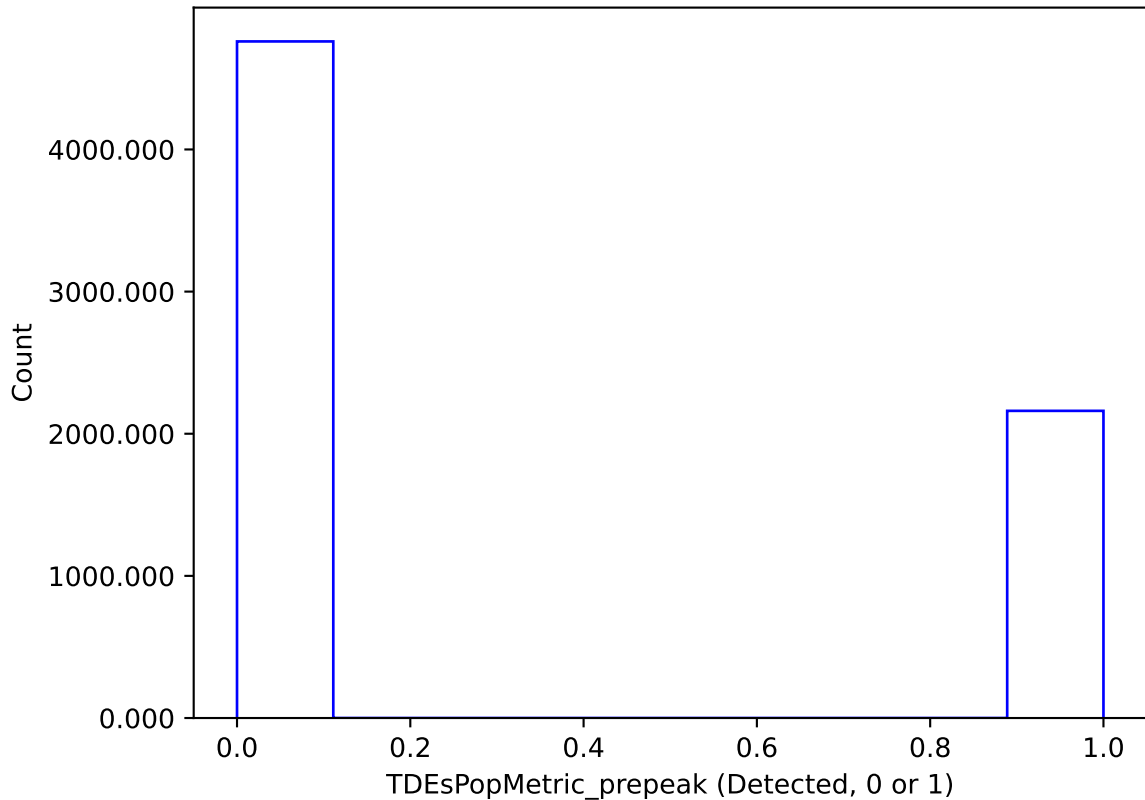
too_elab_r32_d3_giz_v3.4_10yrs : TDEsPopMetric_prepeak
