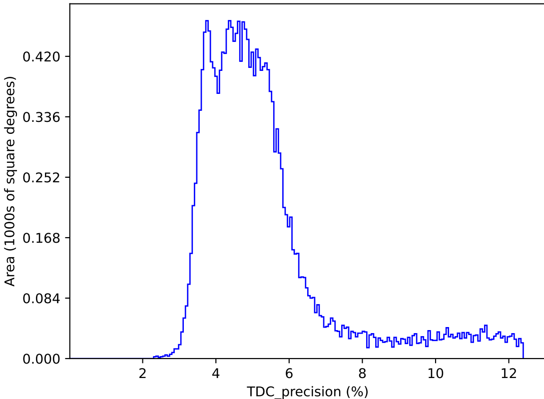
too_elab_r32_d3_giz_v3.4_10yrs : TDC_precision
