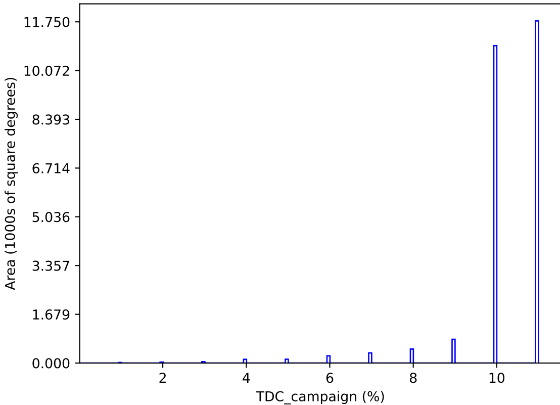
too_elab_r32_d3_giz_v3.4_10yrs : TDC_campaign
