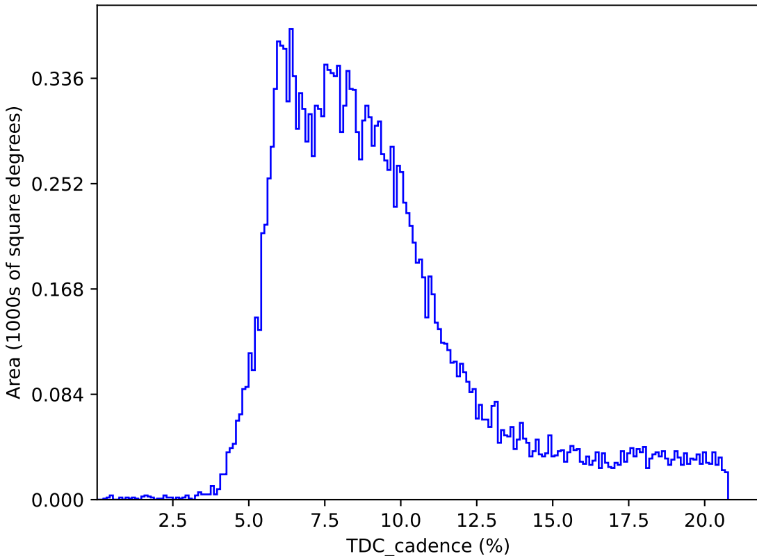
too_elab_r32_d3_giz_v3.4_10yrs : TDC_cadence
