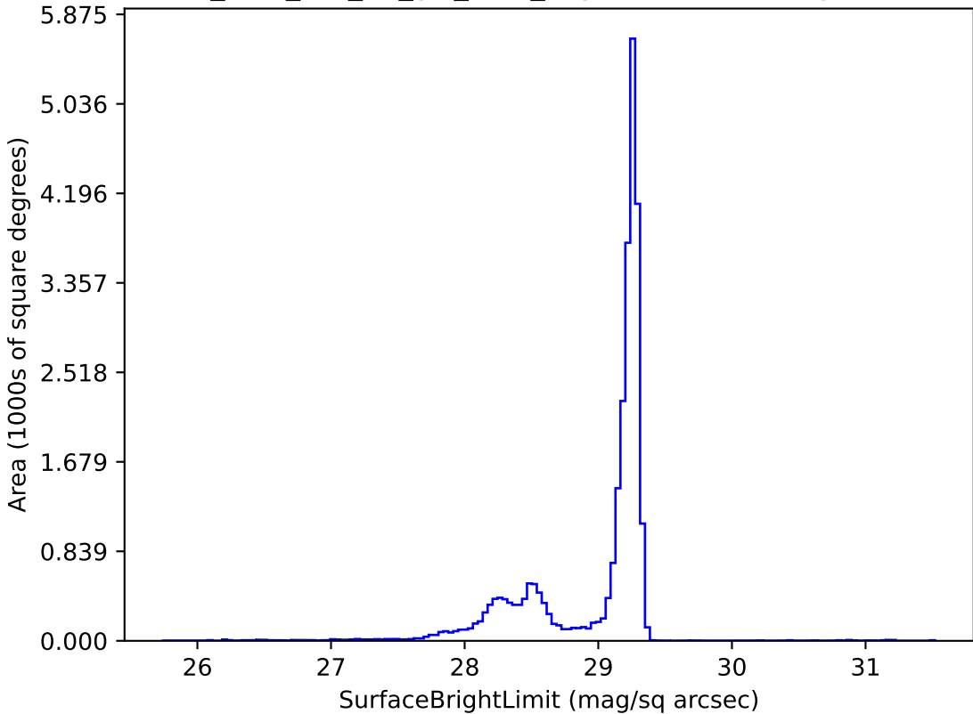
too_elab_r32_d3_giz_v3.4_10yrs z: SurfaceBrightLimit
