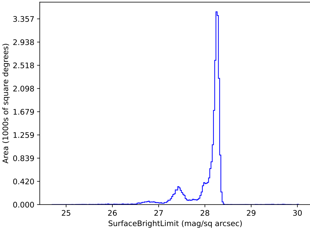
too_elab_r32_d3_giz_v3.4_10yrs y: SurfaceBrightLimit
