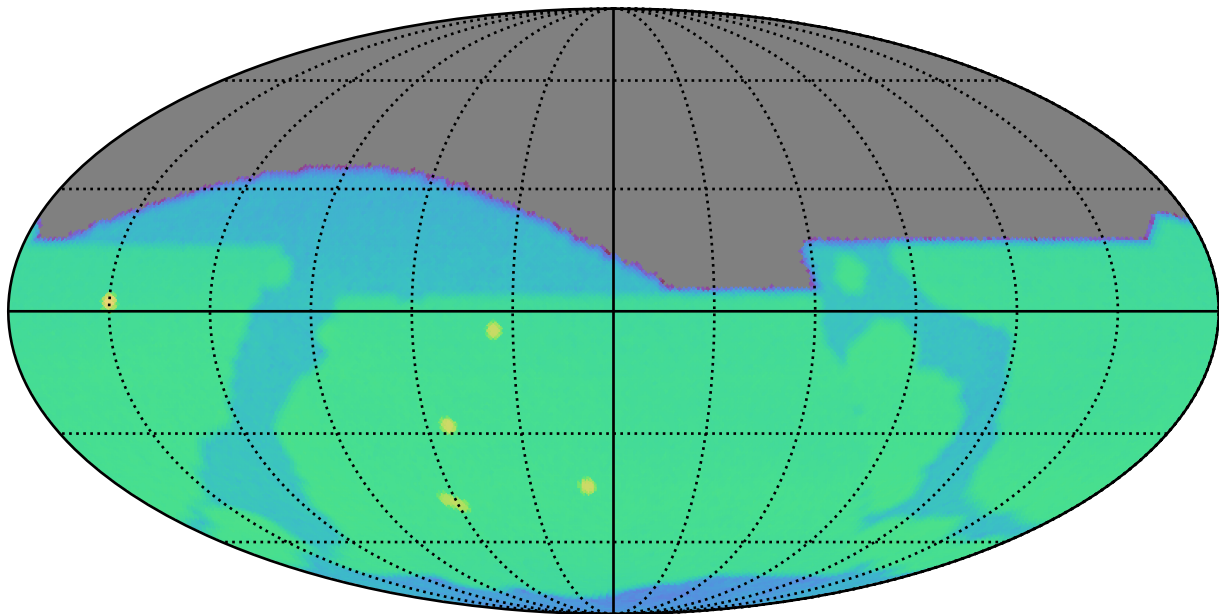
too_elab_r32_d3_giz_v3.4_10yrs r: SurfaceBrightLimit
