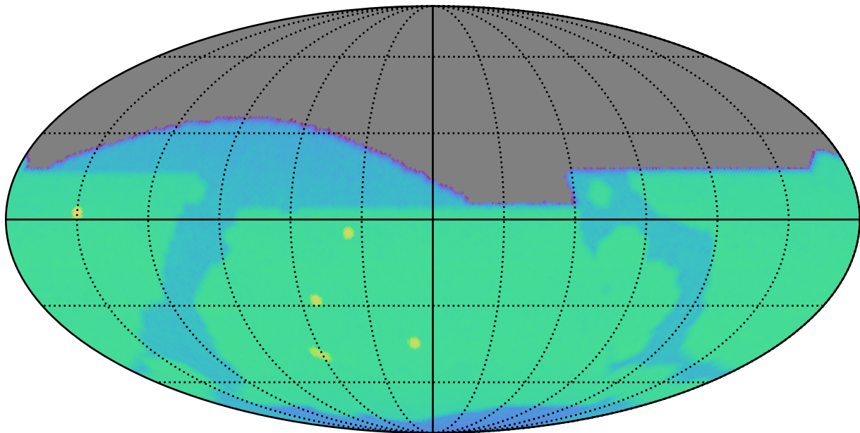
too_elab_r32_d3_giz_v3.4_10yrs i: SurfaceBrightLimit
