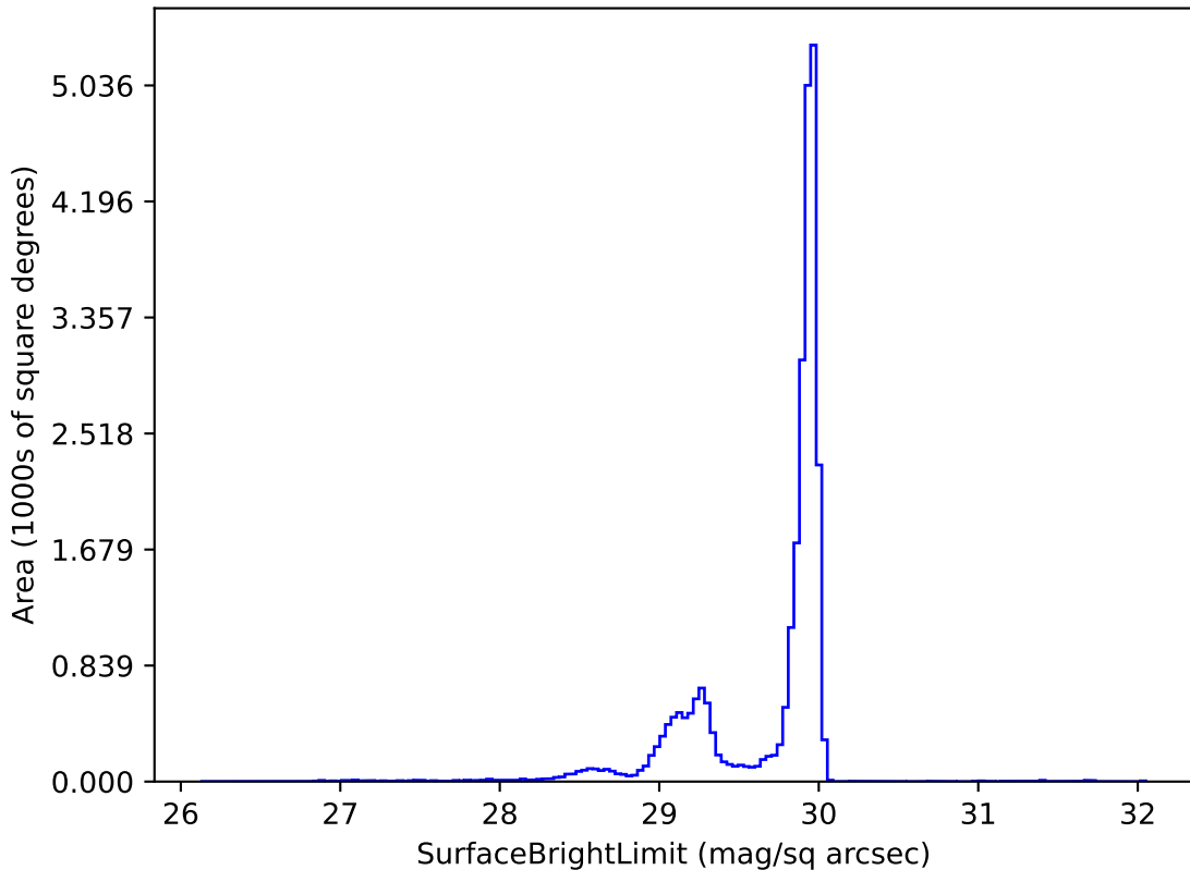
too_elab_r32_d3_giz_v3.4_10yrs i: SurfaceBrightLimit
