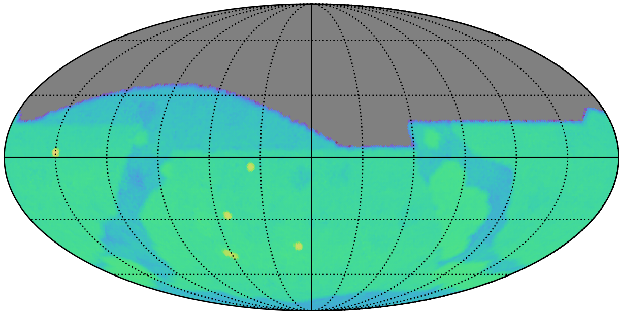
too_elab_r32_d3_giz_v3.4_10yrs g: SurfaceBrightLimit
